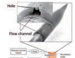
皮膚貼付型生体成分計測用微小流路付金属針と流路断面(針外径200μm) Metal needle with micro flow channel for biological substances monitoring patch Cross-section view of flow channel (needle O.D. 200μm)
