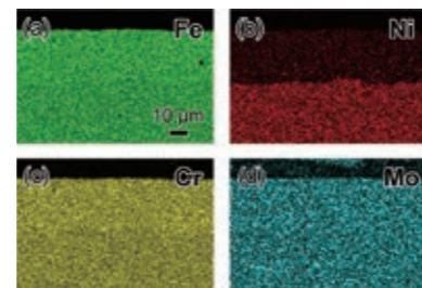
マグネシウム液体中に浸漬してニッケルが除去されたSUS316L表面層断面を示すEDS分析結果 EDS results on cross section of SUS316L surface in which toxic Ni element has been selectively removed in a Mg liquid
