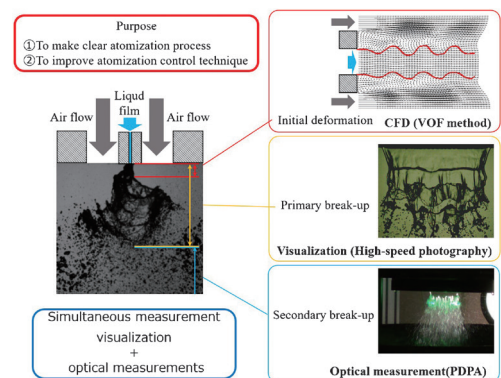
気流による液膜微粒化過程の解明と微粒化制御技術の確立 Elucidation of liquid film atomization process by air flow and establishment of atomization control technology
